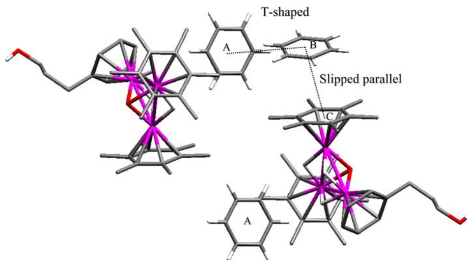
Fig. 4. Capped sticks representation of the \pi interactions in 4 , guest benzene molecules (A), solvate benzene molecule (B) and hexamethylbenzene ligand (C).
